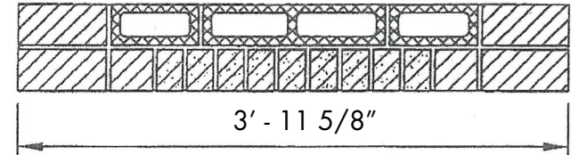
Plan Section
