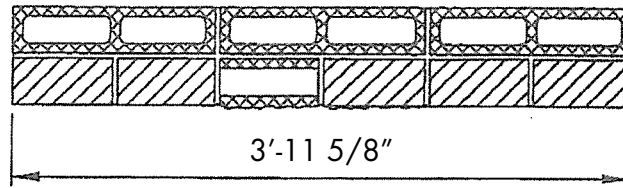
Plan Section
