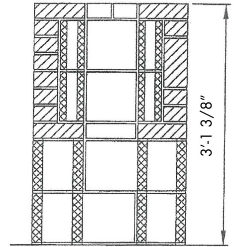
Section
