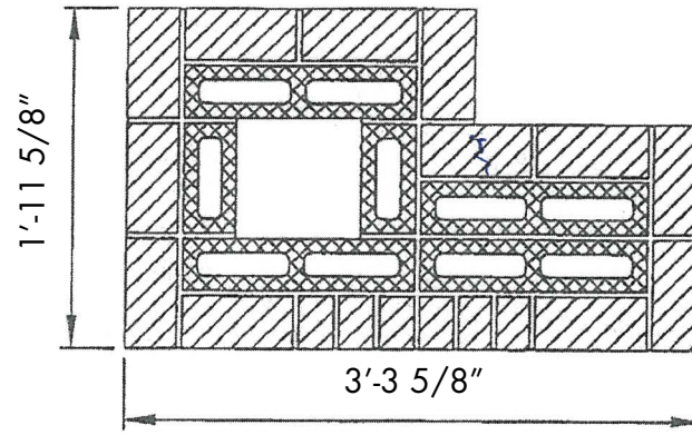
Plan Section
