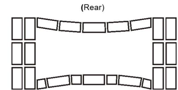
(Rear) 1st and 9th Courses
