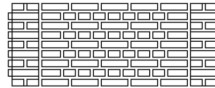
(REAR) English Bond
