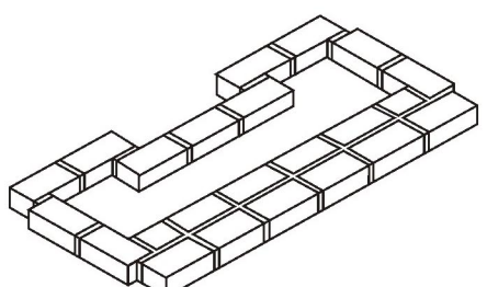
Courses 3 and 9
