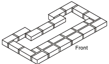
Courses 1 and 11
