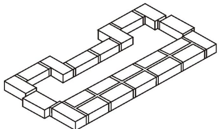
Courses 2 and 10
