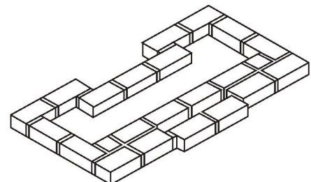
Courses 5 and 7
