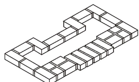
Course No. 6
