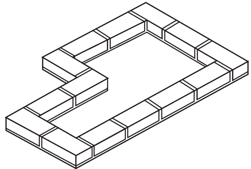
Plan of first course and all odd courses
